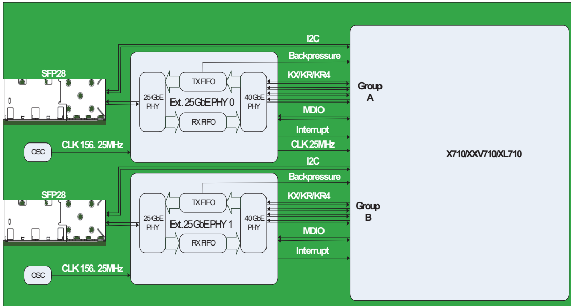
Figure 1-3. Dual-port X710/XXV710/XL710/external 25 GbE PHY configuration
