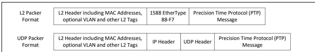
Figure 8-14. 1588 Packet Format
